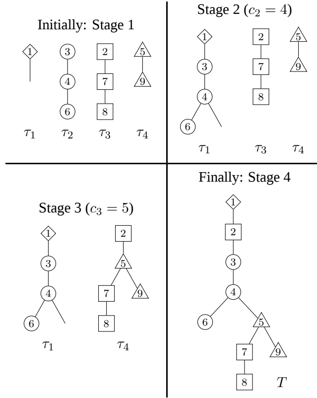
FIGURE 3. Applying \psi_\pi to c = (4, 5) , when \pi has blocks \pi_1 = \{1\} , \pi_2 = \{3, 4, 6\} , \pi_3 = \{2, 7, 8\} , \pi_4 = \{5, 9\} .
