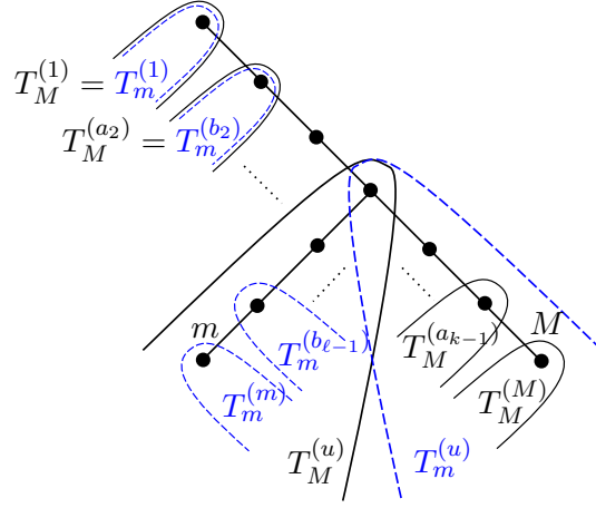
FIGURE 6. M and m decomposition of a tree T ( M -decomposition in black plain lines and m -decomposition in blue dashed lines).
