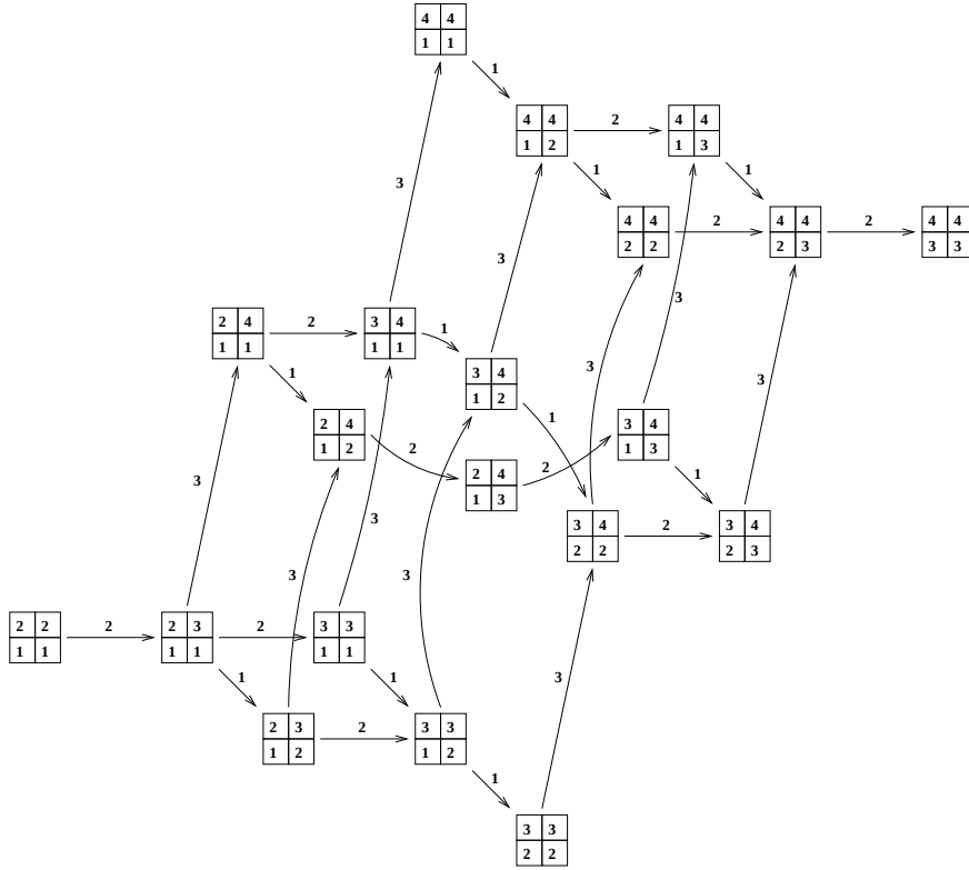
Figure 6.1. The graph structure of the coplactic class of t = 2211 .
