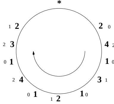
Figure 6.2. The calculation of the cocharge of w = 23141213142 (labels are written in small type)
