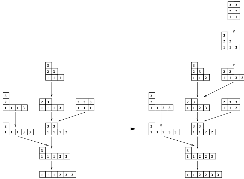
Figure 6.4. The embedding of \text{Tab}(\cdot, (3, 1, 2)) in \text{Tab}(\cdot, (2, 2, 2))
