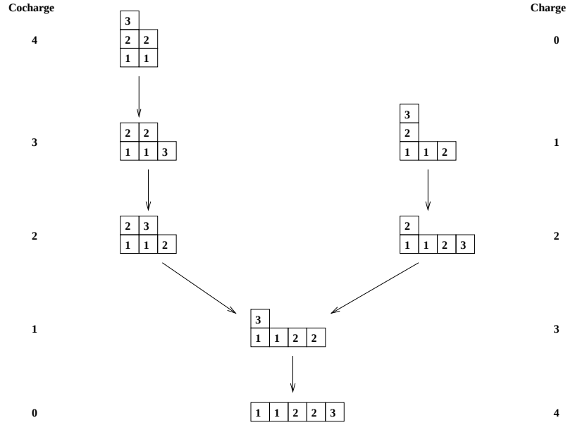
Figure 6.3. The tree structure of \text{Tab}(\cdot, (2, 2, 1))
